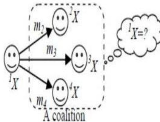
Fig. 1: Data Sharing
