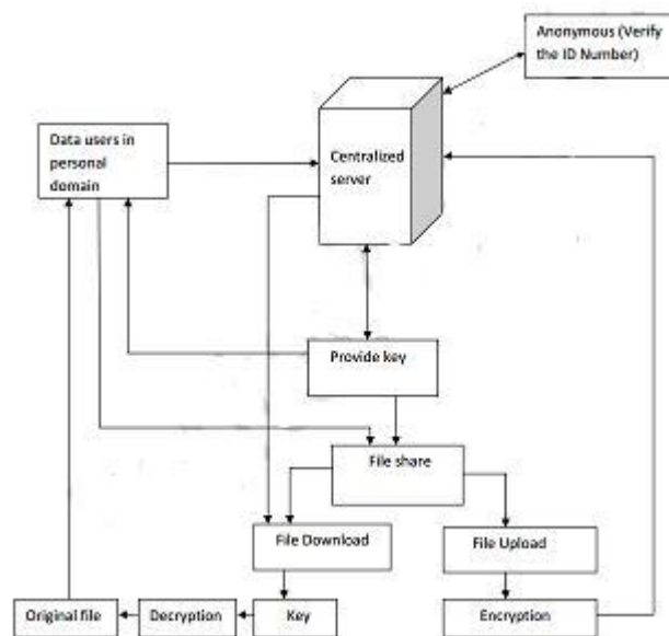
Fig. 2 System Architecture
