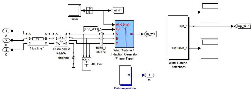
Fig. 2. Simulink diagram of wind farm
